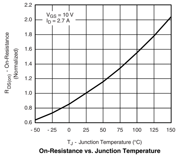
V_{GS} = 10\text{ V} I_D = 2.7\text{ A} T_J - Junction Temperature ( ^\circ\text{C} ) On-Resistance vs. Junction Temperature
