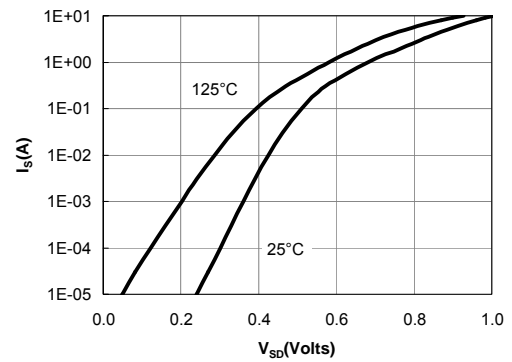
Figure 6: Body-Diode Characteristics
